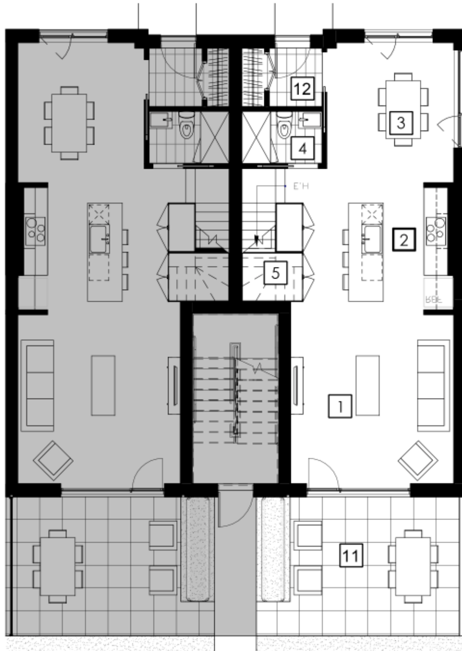
REZ-DE-CHAUSSÉE First Floor
